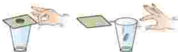
Fig. 8.7: When the card is flicked with the finger the coin placed over it falls in the tumbler.
