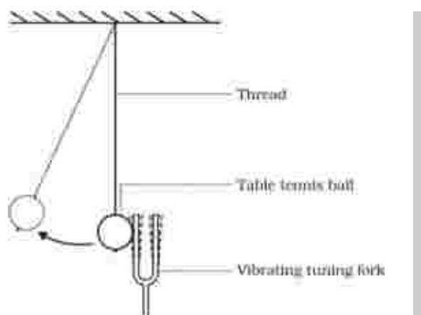
Fig. 11.1: Vibrating tuning fork just touching the suspended table tennis ball.
